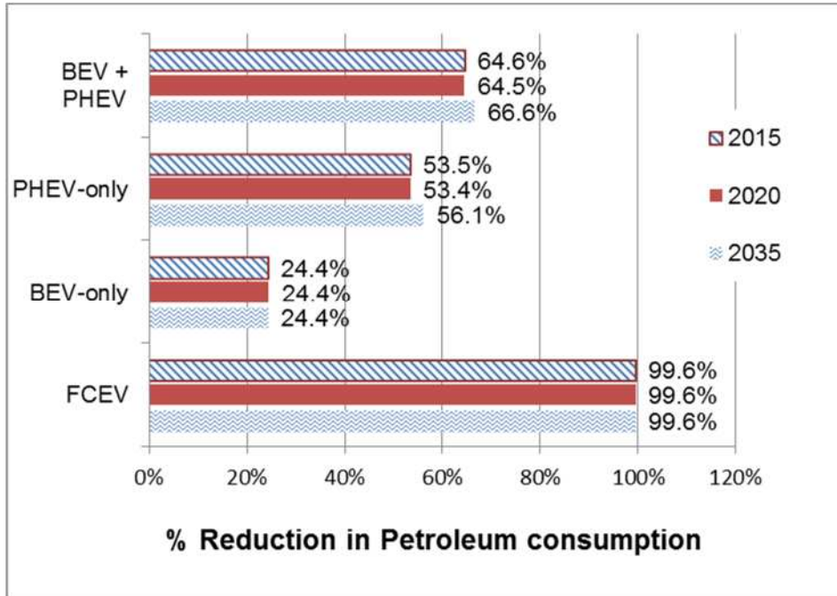
Figure 5. Calculated reductions in petroleum use (large is good!) for the four vehicle scenarios and three time periods
